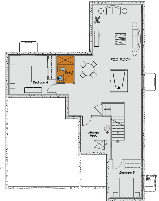
OPTION 1 EXT. FINISHED BASEMENT PLAN AT ELEVATION 'A' SIMILAR AT ELEVATION 'B' & 'C'
