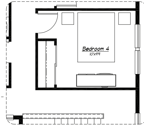
(Optional) Bedroom 4
