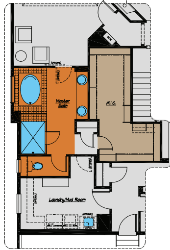
2,458 SQ.FT. (Opt.) Expanded Master Suite and Laundry
